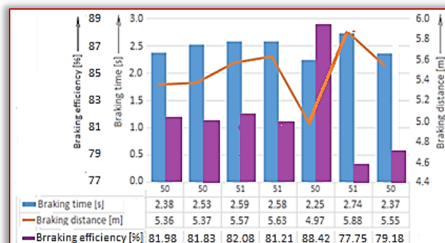
Figure 7. Braking time, distance, and efficiency based on vehicle speed (50–51 km/h)
